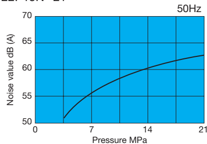
NNP-30-37P22N*-21
