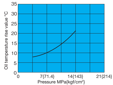
NNP-30-37P22N*-21
